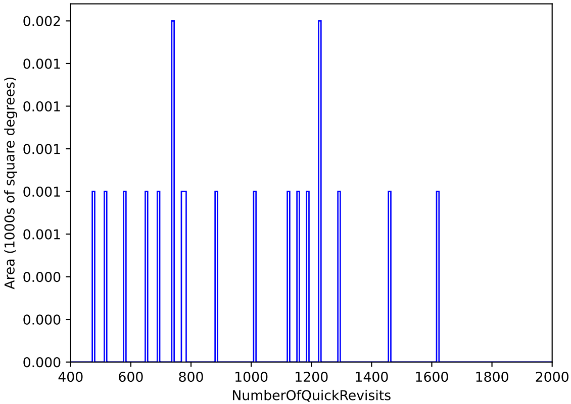
too_elab_r128_d2_griz_v3.4_10yrs WFD: NumberOfQuickRevisits
