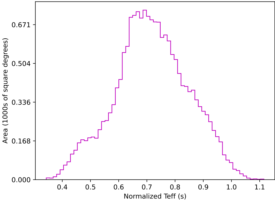
too_elab_r128_d2_griz_v3.4_10yrs WFD z band: Normalized Teff
