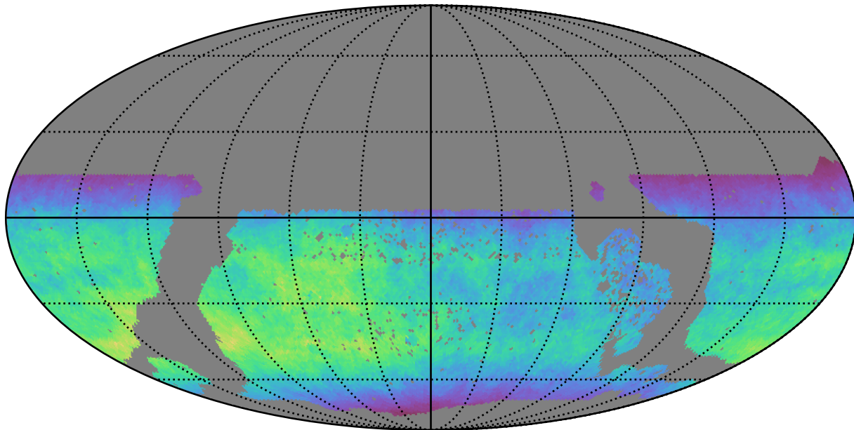
too_elab_r128_d2_griz_v3.4_10yrs WFD y band: Normalized Teff
