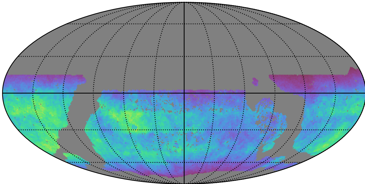
too_elab_r128_d2_griz_v3.4_10yrs WFD u band: Normalized Teff
