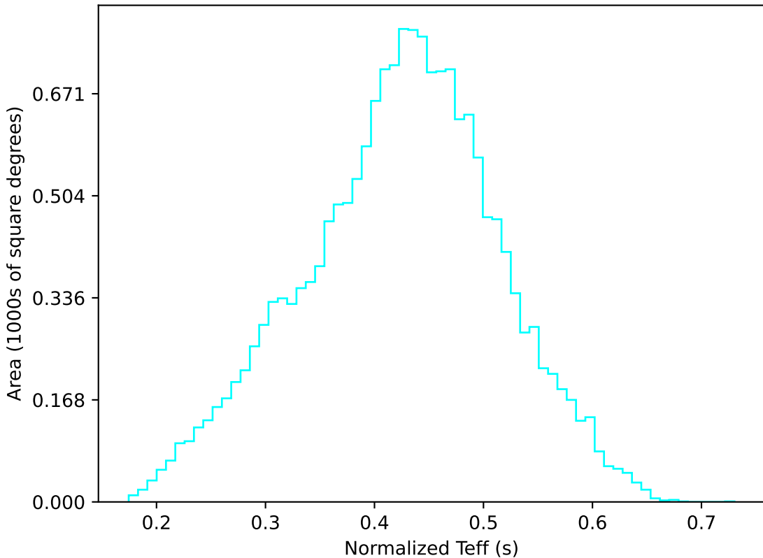
too_elab_r128_d2_griz_v3.4_10yrs WFD u band: Normalized Teff
