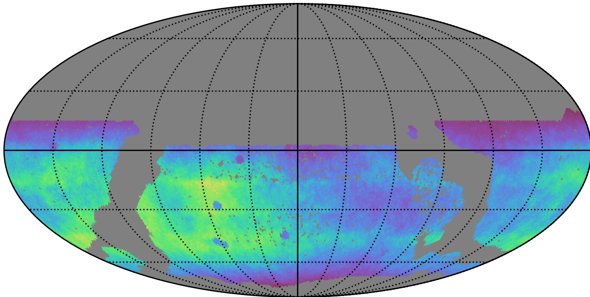
too_elab_r128_d2_griz_v3.4_10yrs WFD r band: Normalized Teff
