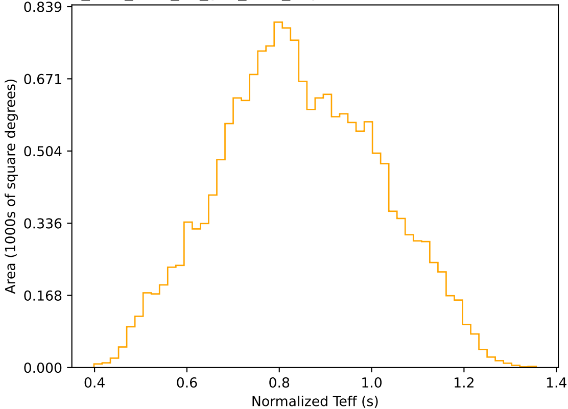
too_elab_r128_d2_griz_v3.4_10yrs WFD r band: Normalized Teff
