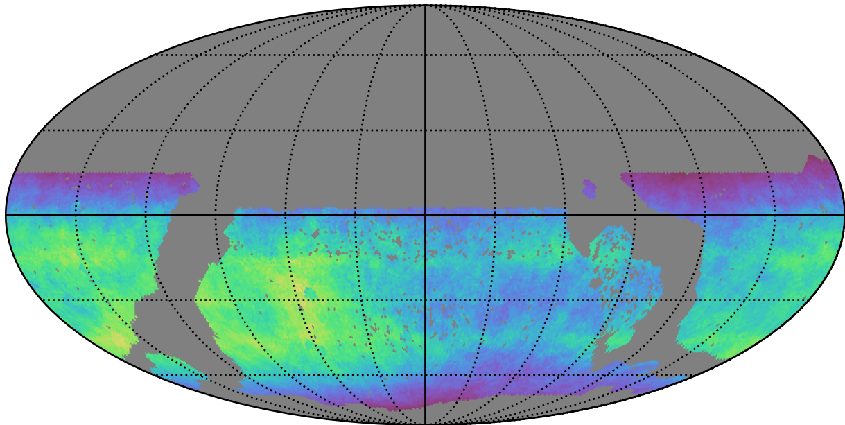
too_elab_r128_d2_griz_v3.4_10yrs WFD i band: Normalized Teff
