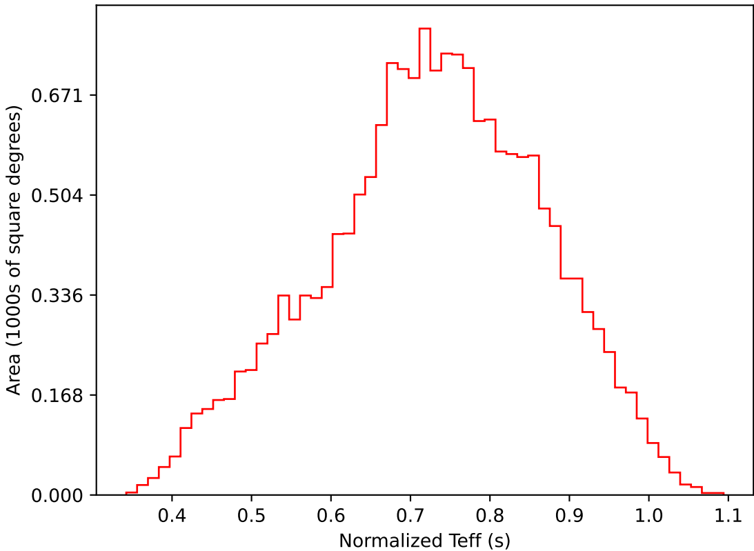
too_elab_r128_d2_griz_v3.4_10yrs WFD i band: Normalized Teff
