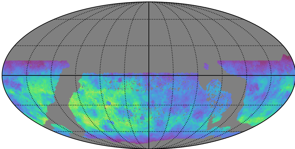
too_elab_r128_d2_griz_v3.4_10yrs WFD g band: Normalized Teff
