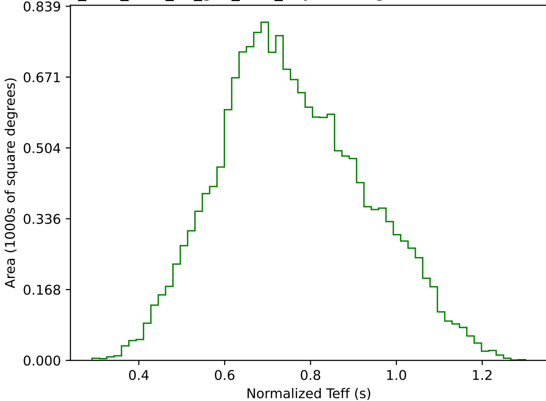
too_elab_r128_d2_griz_v3.4_10yrs WFD g band: Normalized Teff
