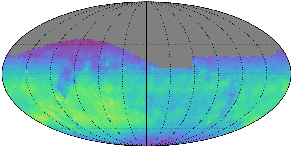
too_elab_r128_d2_griz_v3.4_10yrs All sky z band: Normalized Teff
