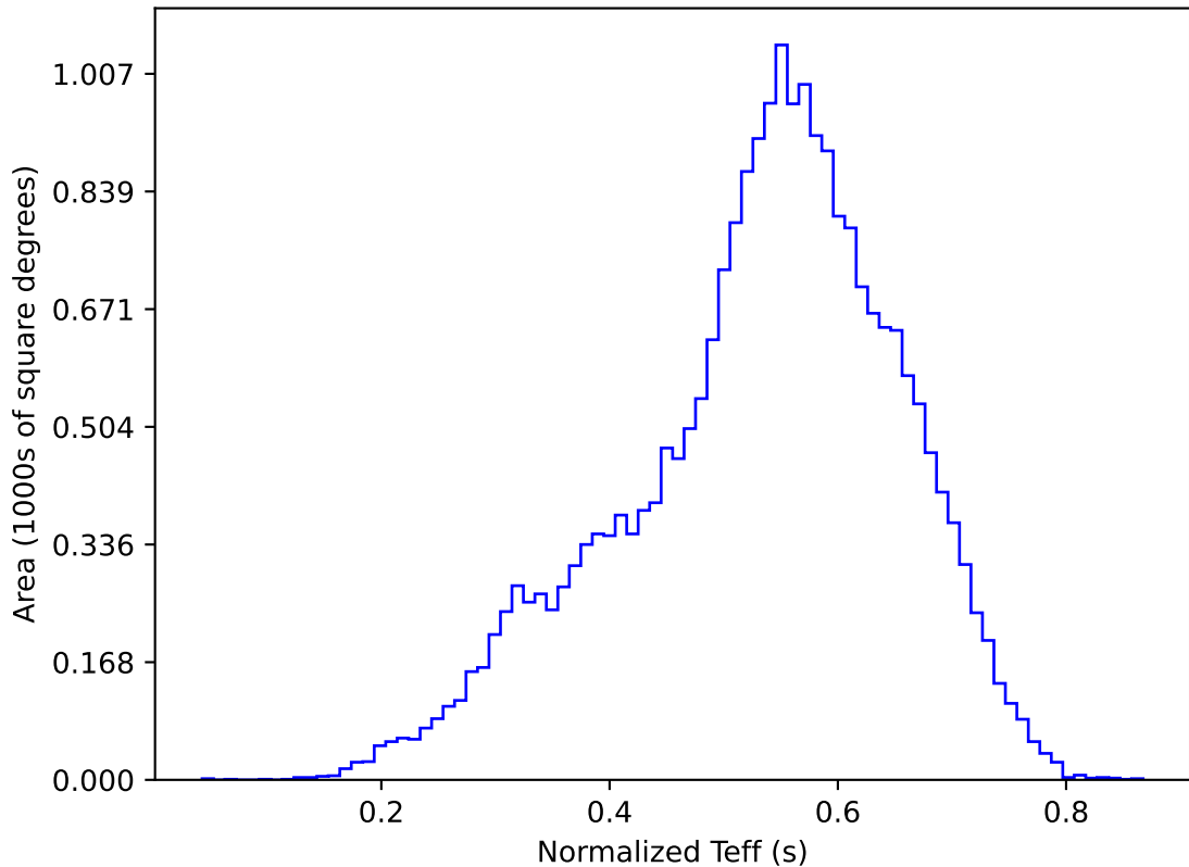
too_elab_r128_d2_griz_v3.4_10yrs All sky y band: Normalized Teff
