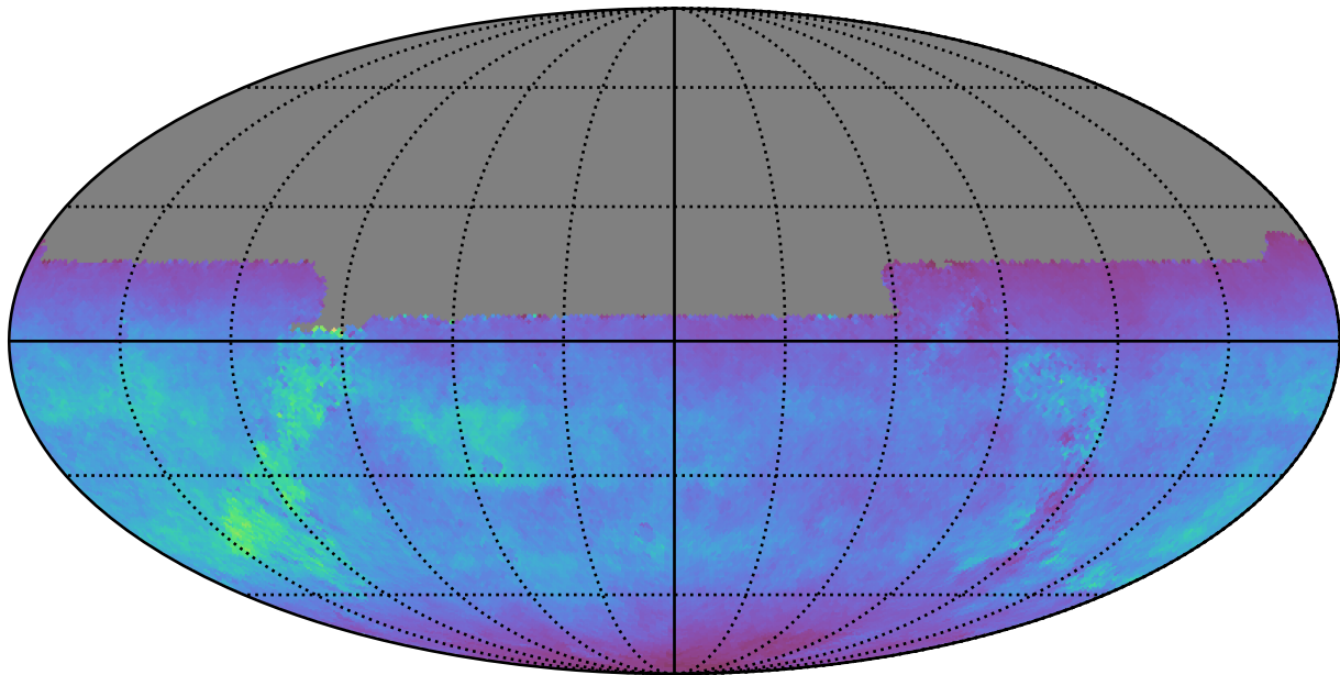
too_elab_r128_d2_griz_v3.4_10yrs All sky u band: Normalized Teff
