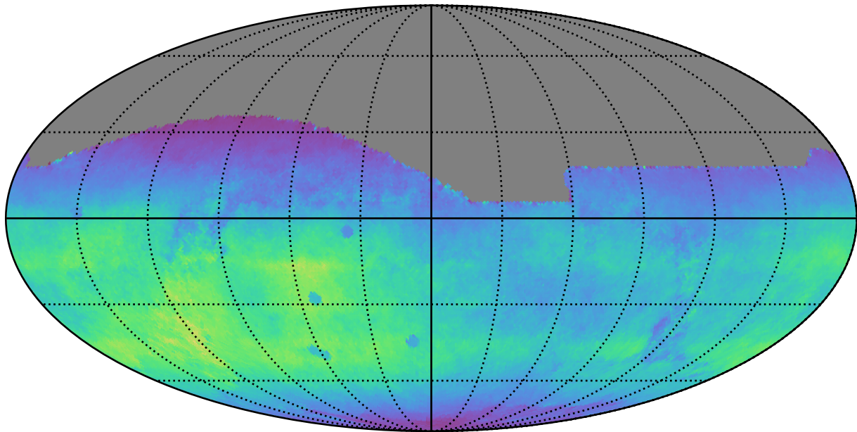
too_elab_r128_d2_griz_v3.4_10yrs All sky r band: Normalized Teff
