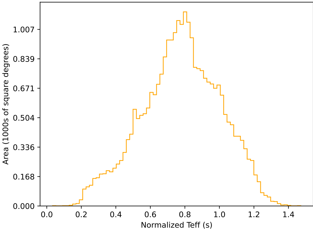
too_elab_r128_d2_griz_v3.4_10yrs All sky r band: Normalized Teff
