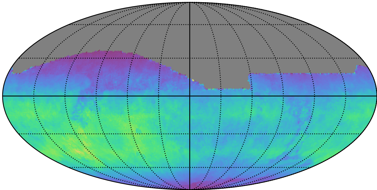
too_elab_r128_d2_griz_v3.4_10yrs All sky i band: Normalized Teff
