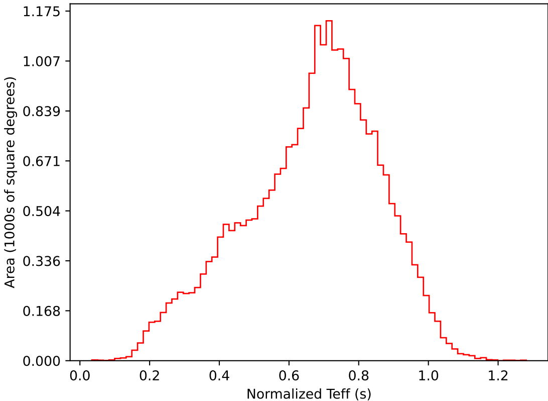
too_elab_r128_d2_griz_v3.4_10yrs All sky i band: Normalized Teff
