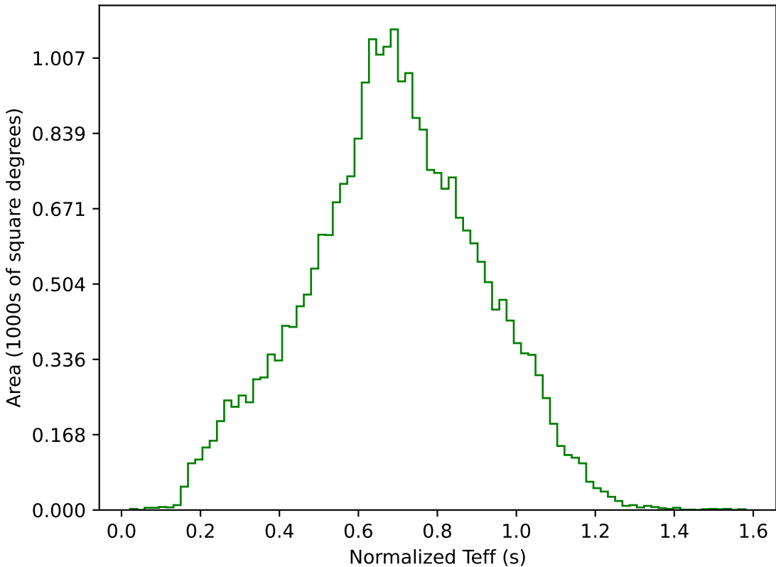
too_elab_r128_d2_griz_v3.4_10yrs All sky g band: Normalized Teff
