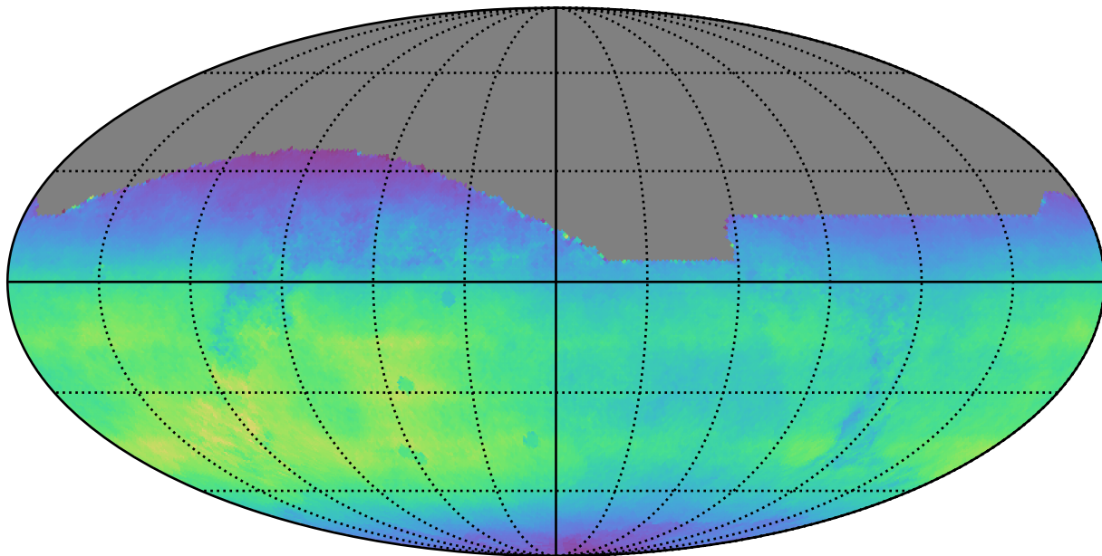
too_elab_r128_d2_griz_v3.4_10yrs All sky all bands: Normalized Teff
