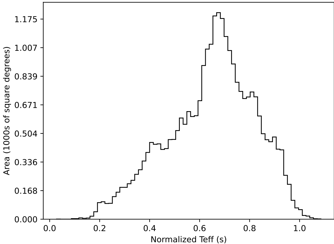
too_elab_r128_d2_griz_v3.4_10yrs All sky all bands: Normalized Teff
