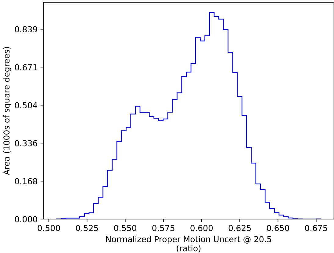
too_elab_r128_d2_griz_v3.4_10yrs WFD: Normalized Proper Motion Uncert @ 20.5
