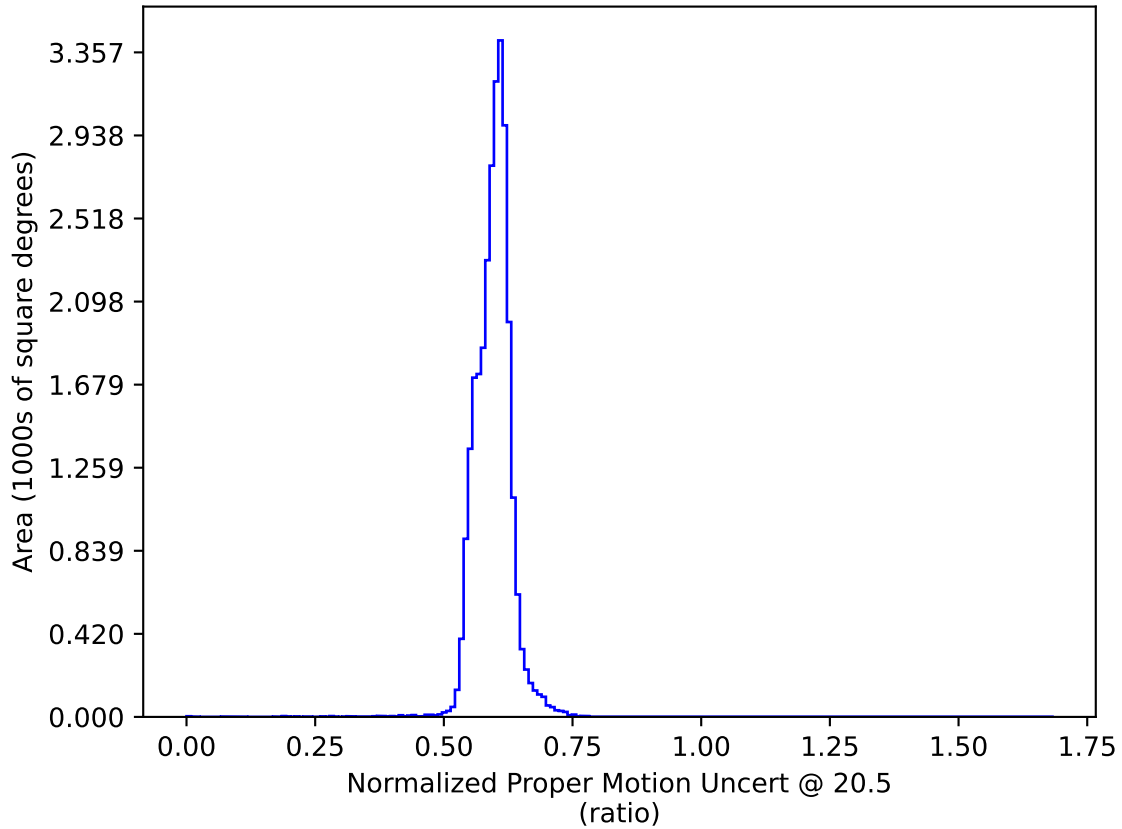
too_elab_r128_d2_griz_v3.4_10yrs All sky: Normalized Proper Motion Uncert @ 20.5
