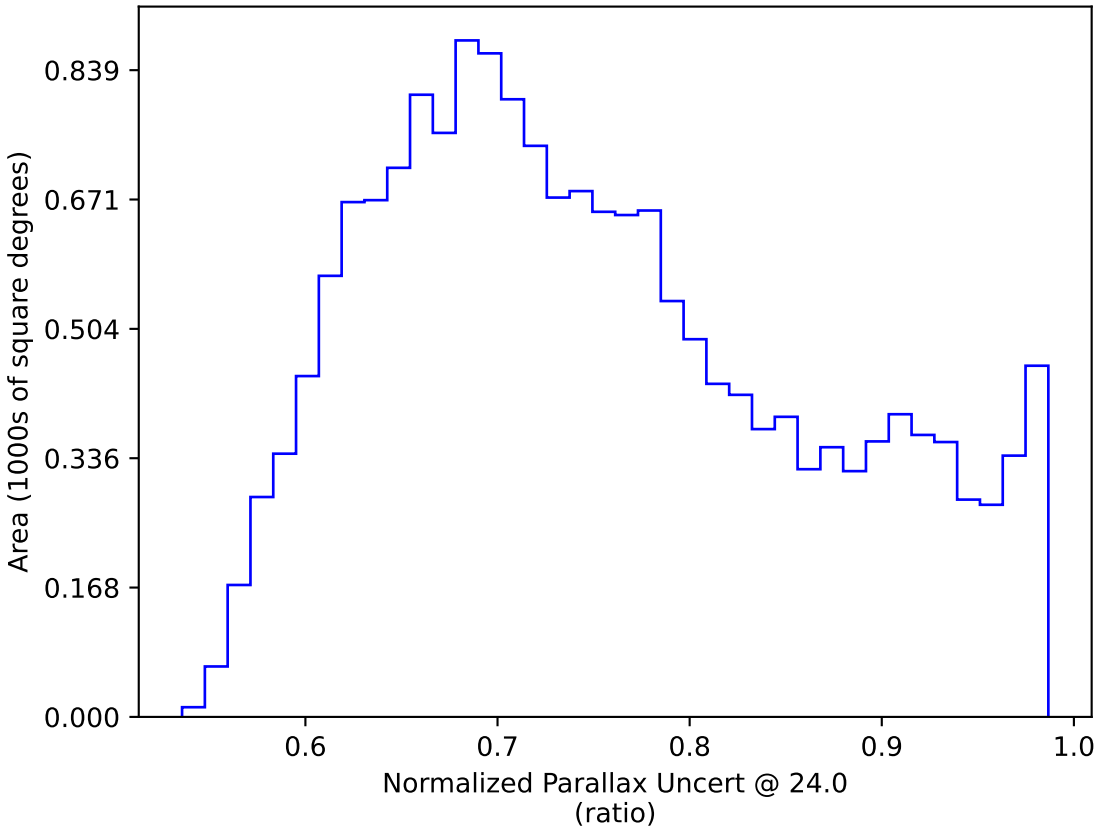
too_elab_r128_d2_griz_v3.4_10yrs WFD: Normalized Parallax Uncert @ 24.0
