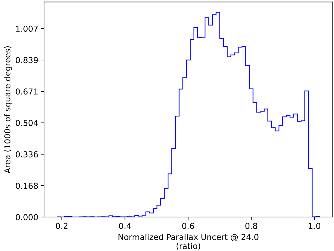
too_elab_r128_d2_griz_v3.4_10yrs All sky: Normalized Parallax Uncert @ 24.0
