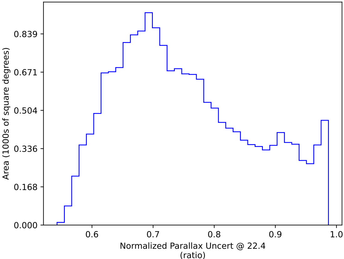
too_elab_r128_d2_griz_v3.4_10yrs WFD: Normalized Parallax Uncert @ 22.4
