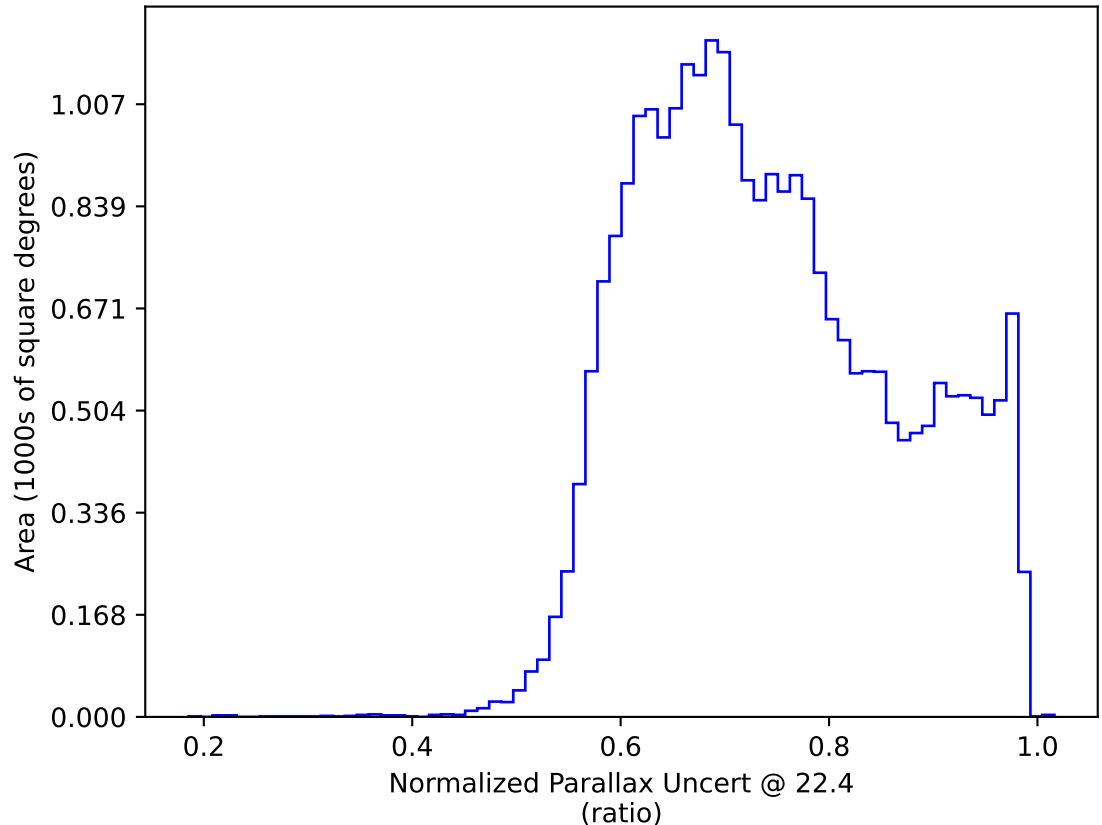
too_elab_r128_d2_griz_v3.4_10yrs All sky: Normalized Parallax Uncert @ 22.4
