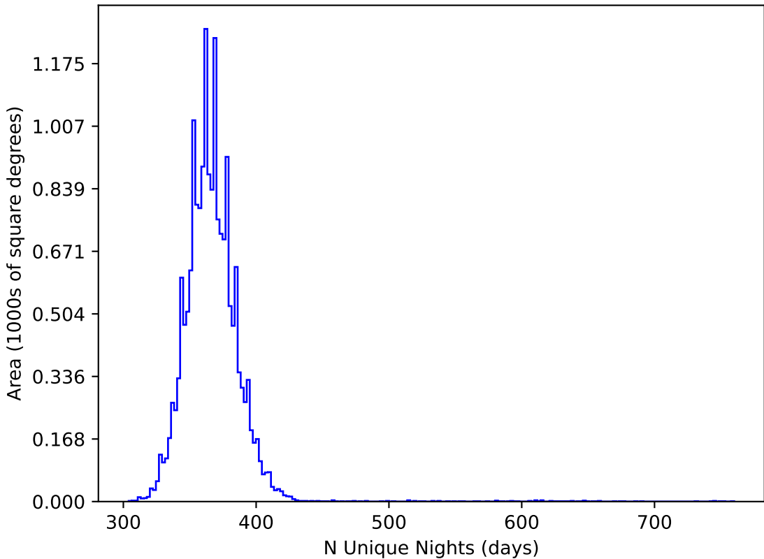
too_elab_r128_d2_griz_v3.4_10yrs WFD all bands: N Unique Nights
