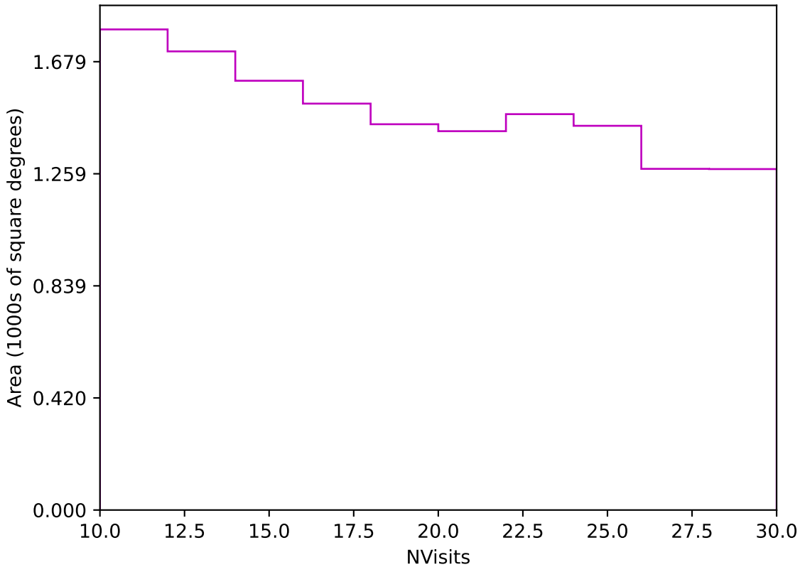
too_elab_r128_d2_griz_v3.4_10yrs Yr 3-4 z band: NVisits
