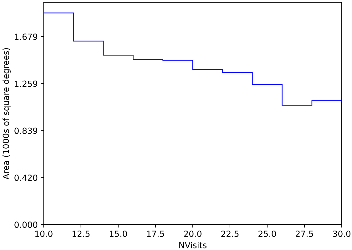
too_elab_r128_d2_griz_v3.4_10yrs Yr 3-4 y band: NVisits
