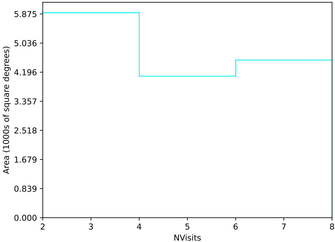
too_elab_r128_d2_griz_v3.4_10yrs Yr 3-4 u band: NVisits
