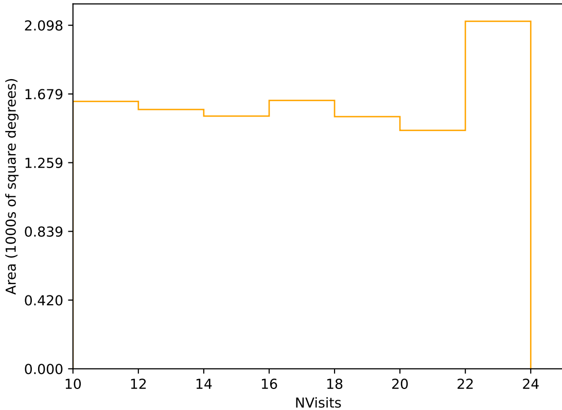
too_elab_r128_d2_griz_v3.4_10yrs Yr 3-4 r band: NVisits
