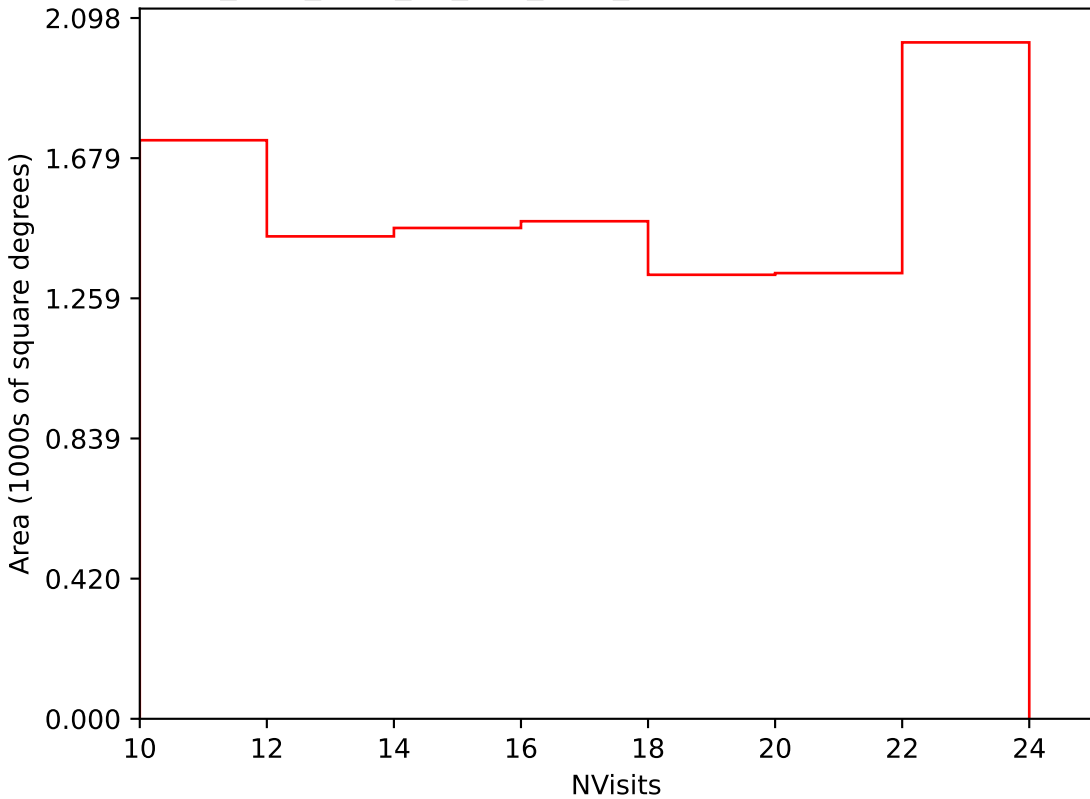
too_elab_r128_d2_griz_v3.4_10yrs Yr 3-4 i band: NVisits
