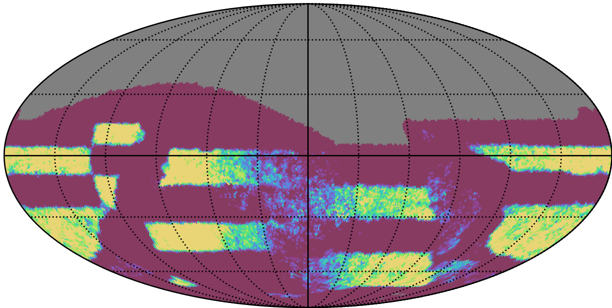
too_elab_r128_d2_griz_v3.4_10yrs Yr 3-4 all bands: NVisits
