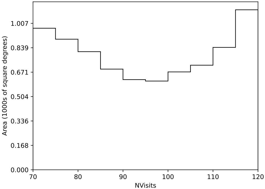
too_elab_r128_d2_griz_v3.4_10yrs Yr 3-4 all bands: NVisits
