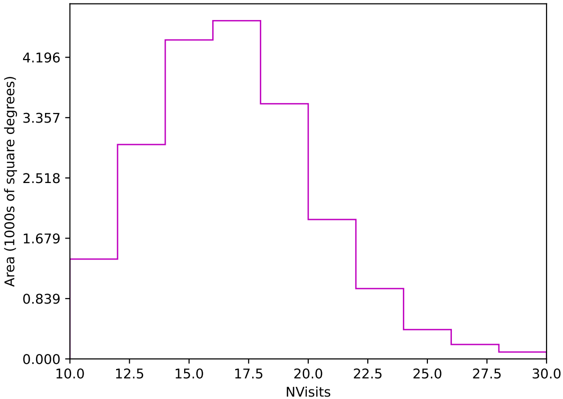
too_elab_r128_d2_griz_v3.4_10yrs Yr 1 z band: NVisits
