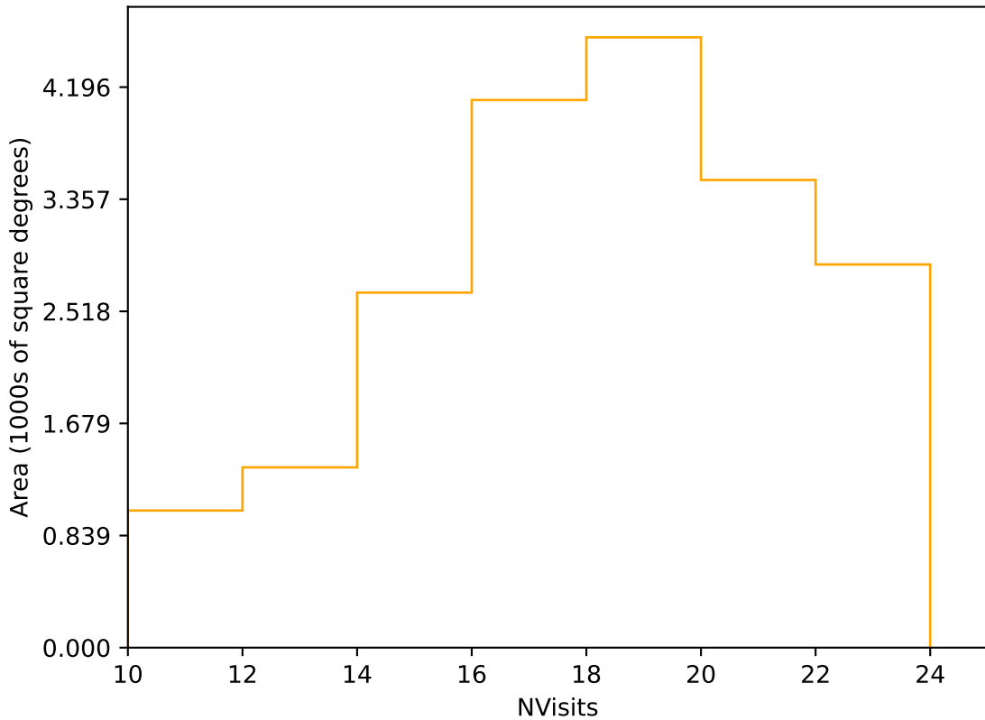
too_elab_r128_d2_griz_v3.4_10yrs Yr 1 r band: NVisits
