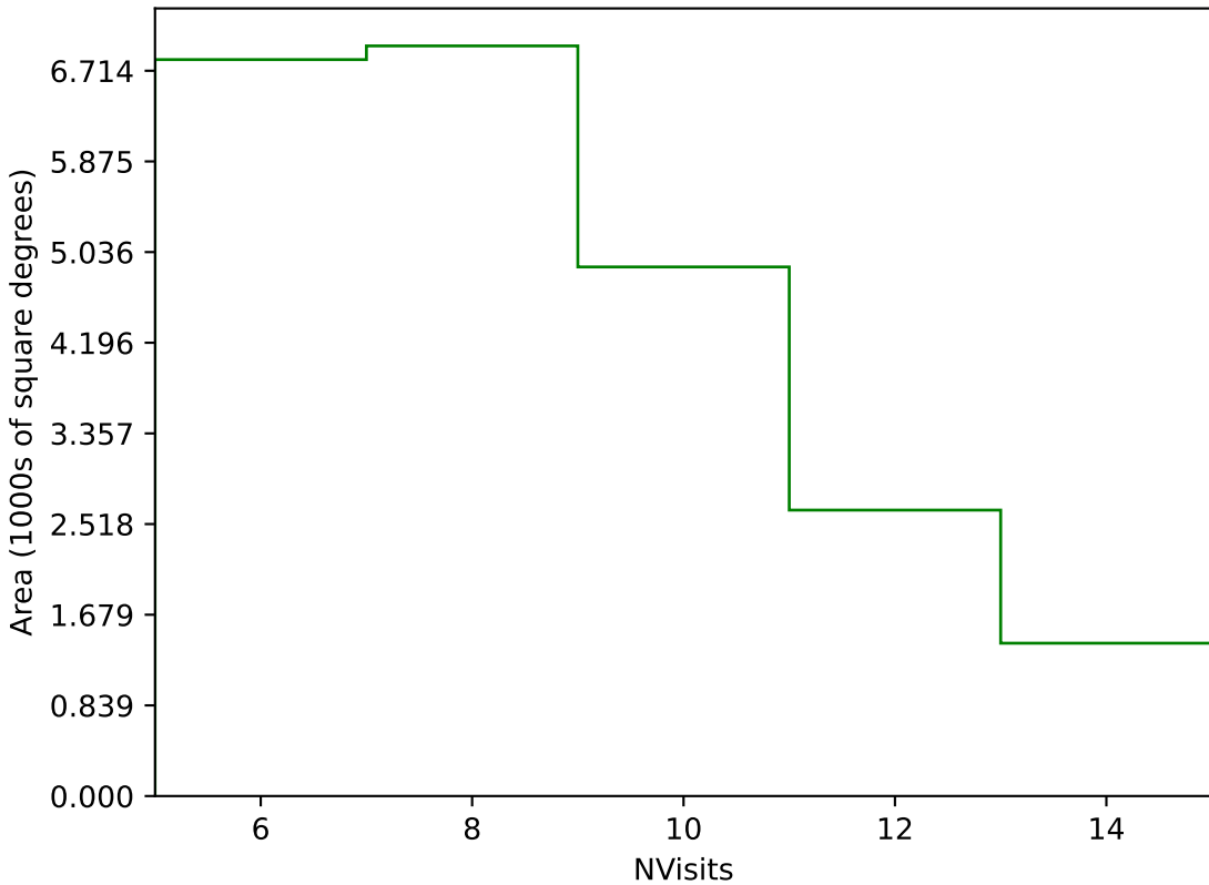
too_elab_r128_d2_griz_v3.4_10yrs Yr 1 g band: NVisits
