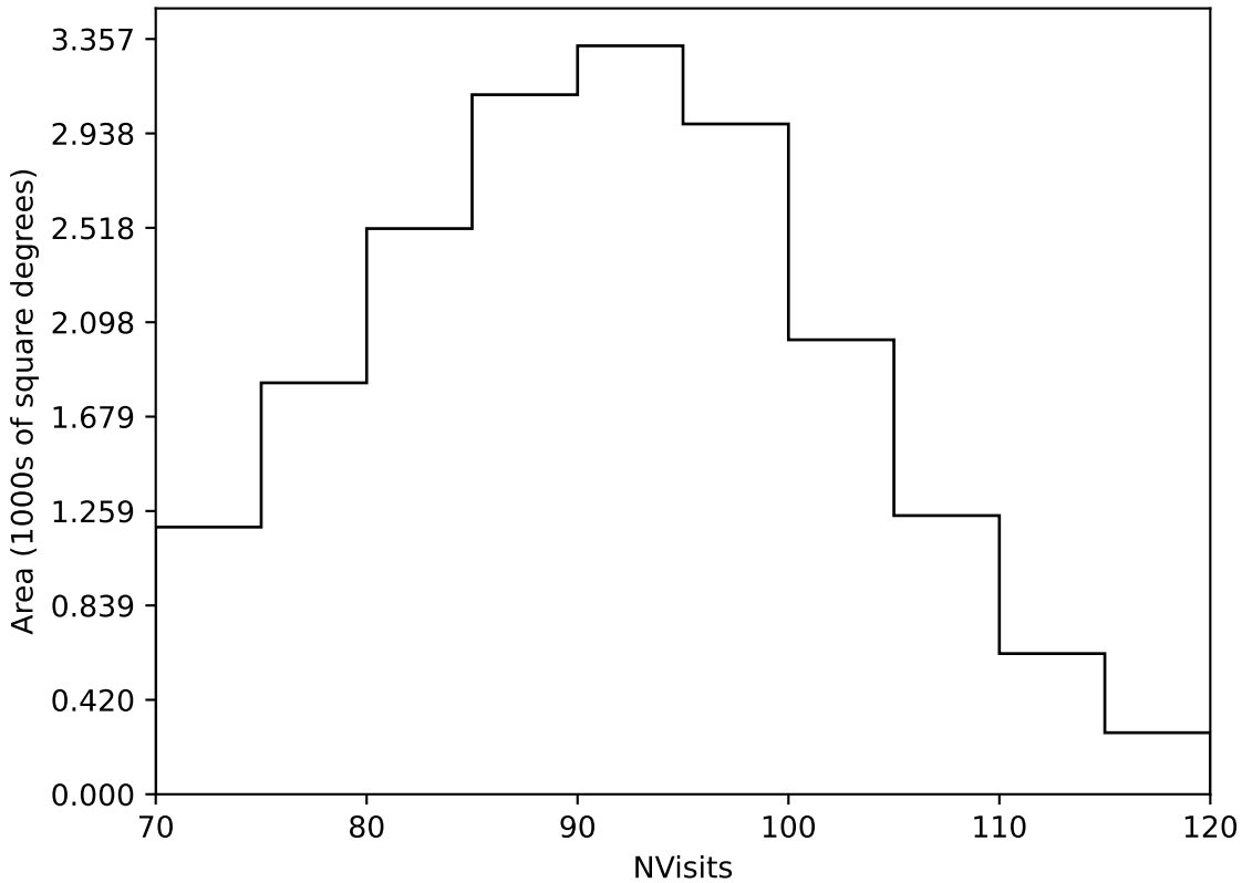
too_elab_r128_d2_griz_v3.4_10yrs Yr 1 all bands: NVisits
