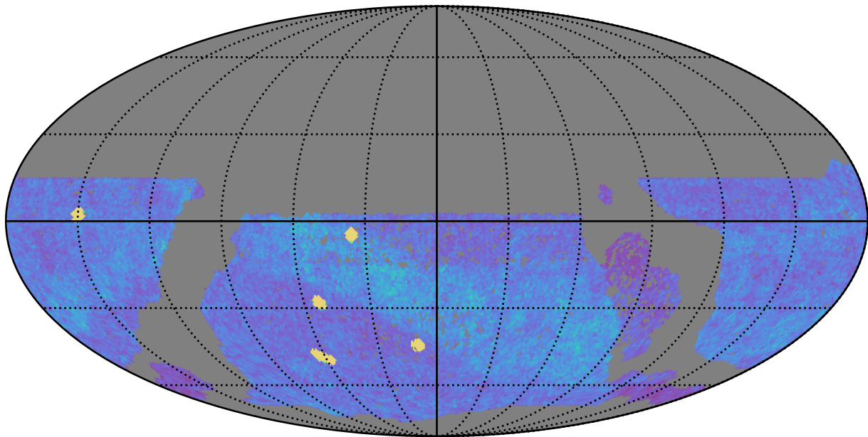
too_elab_r128_d2_griz_v3.4_10yrs WFD z band: NVisits
