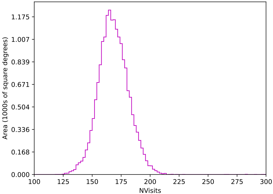
too_elab_r128_d2_griz_v3.4_10yrs WFD z band: NVisits
