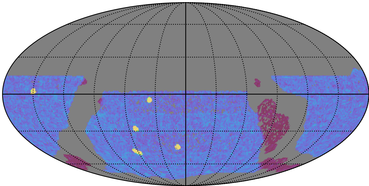
too_elab_r128_d2_griz_v3.4_10yrs WFD y band: NVisits
