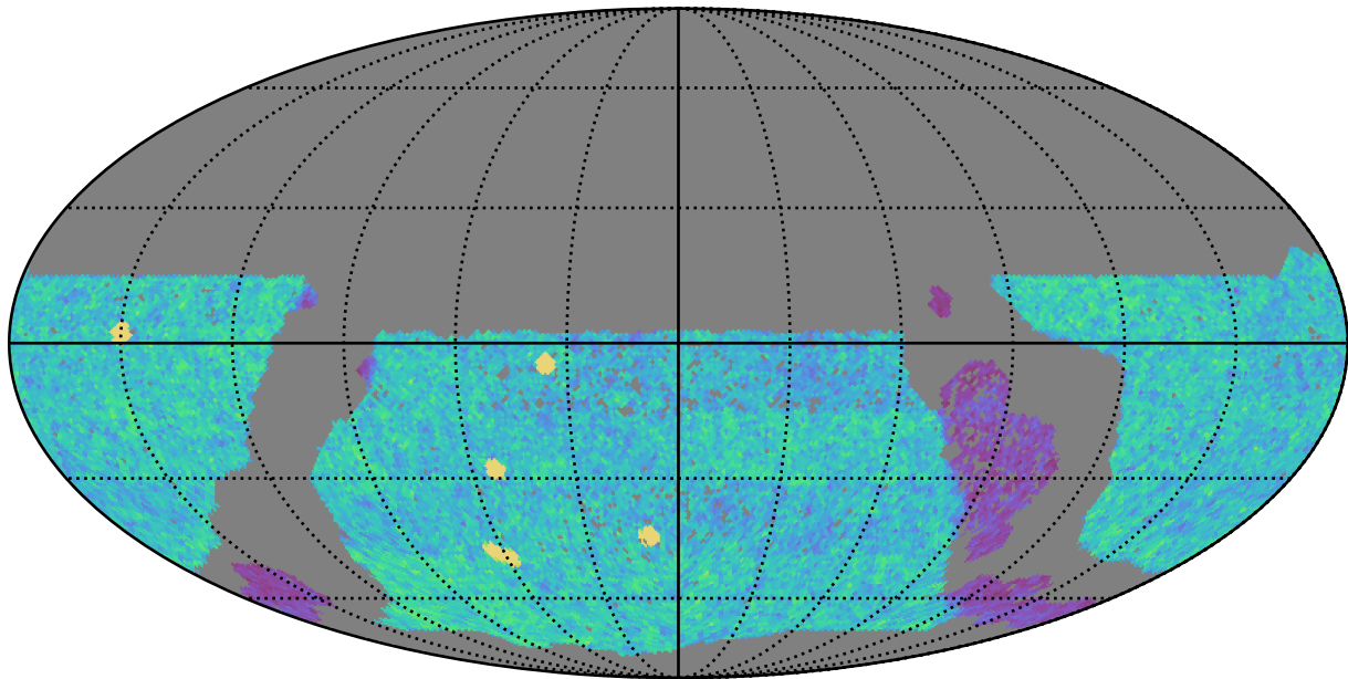
too_elab_r128_d2_griz_v3.4_10yrs WFD u band: NVisits
