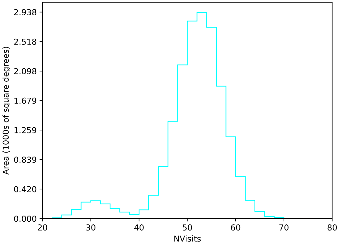
too_elab_r128_d2_griz_v3.4_10yrs WFD u band: NVisits
