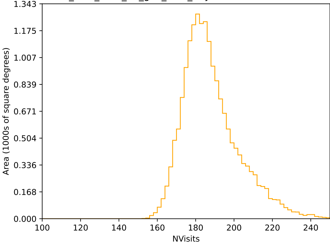
too_elab_r128_d2_griz_v3.4_10yrs WFD r band: NVisits
