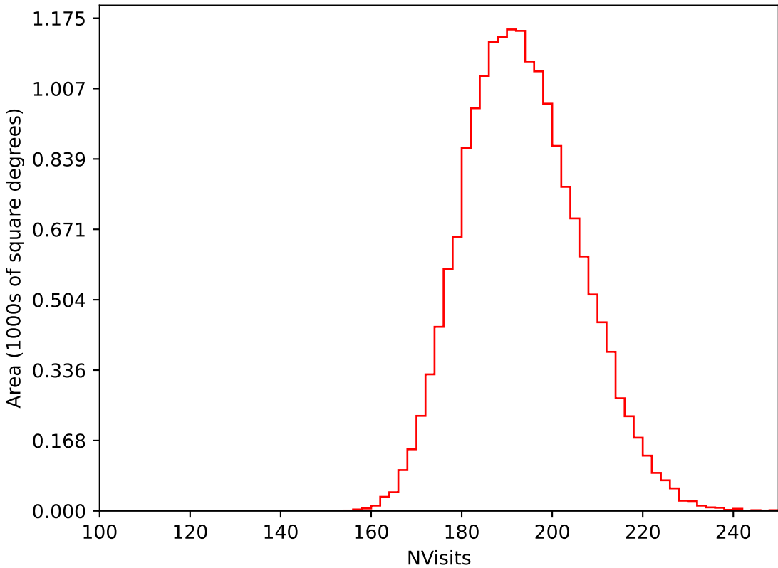
too_elab_r128_d2_griz_v3.4_10yrs WFD i band: NVisits
