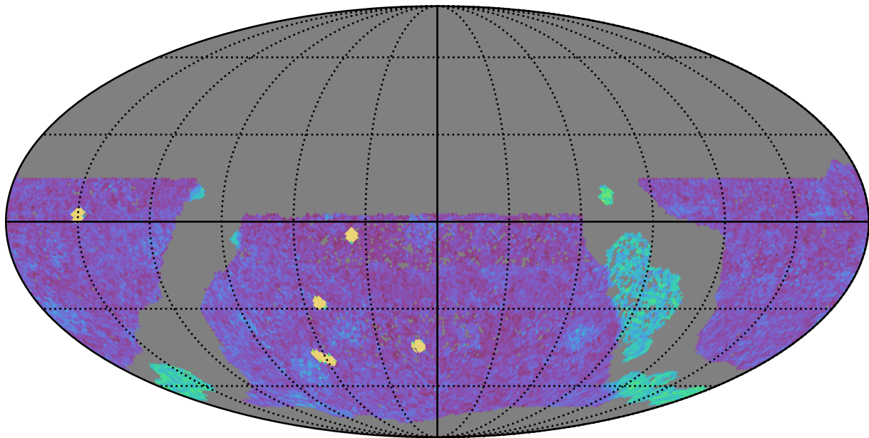
too_elab_r128_d2_griz_v3.4_10yrs WFD g band: NVisits
