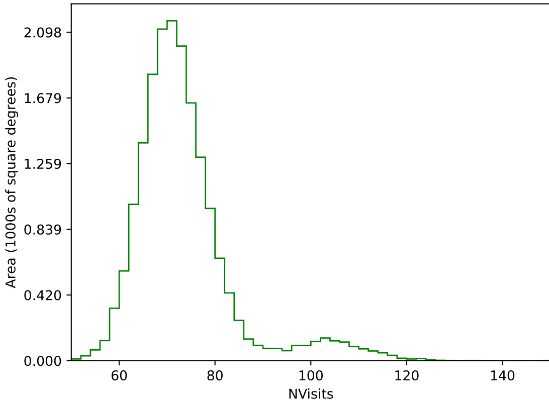
too_elab_r128_d2_griz_v3.4_10yrs WFD g band: NVisits
