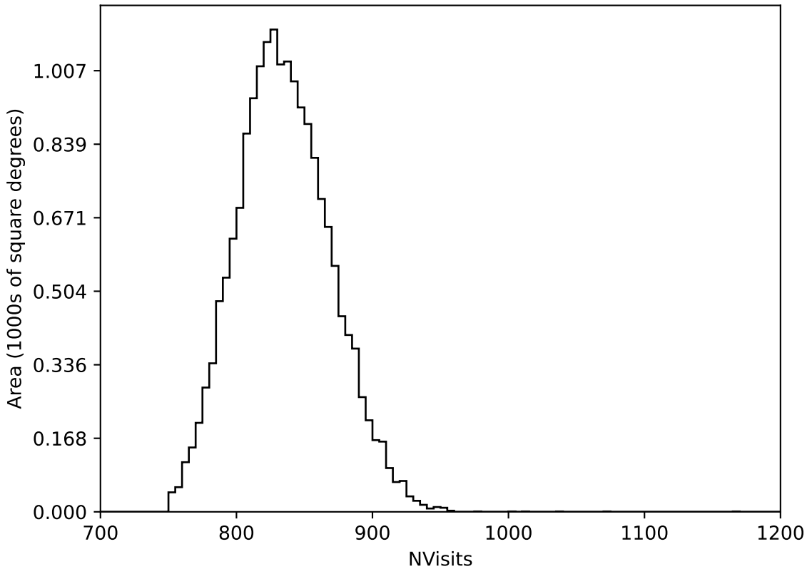
too_elab_r128_d2_griz_v3.4_10yrs WFD all bands: NVisits
