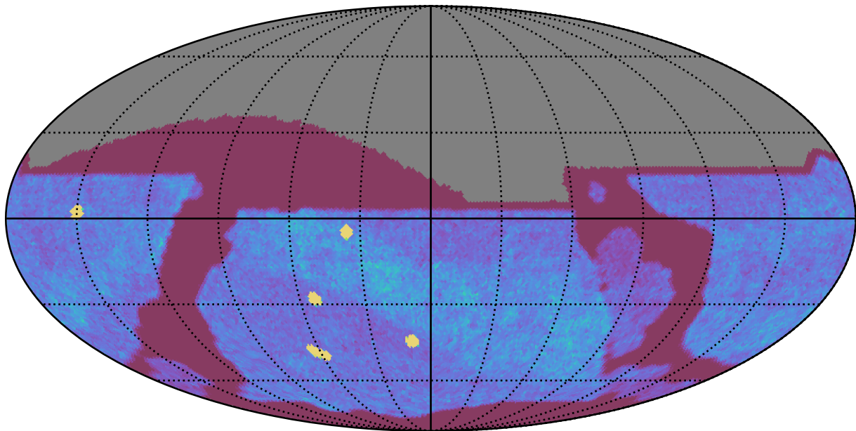
too_elab_r128_d2_griz_v3.4_10yrs All sky z band: NVisits
